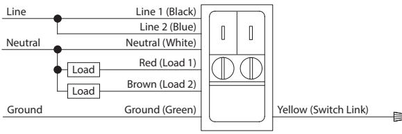
VS 2 Basic Wiring
